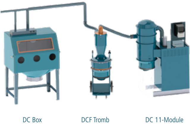
Installation example for our DC Box.
