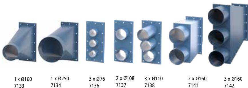
Inlet modules for F 20000 and F 30000 (Part No)
