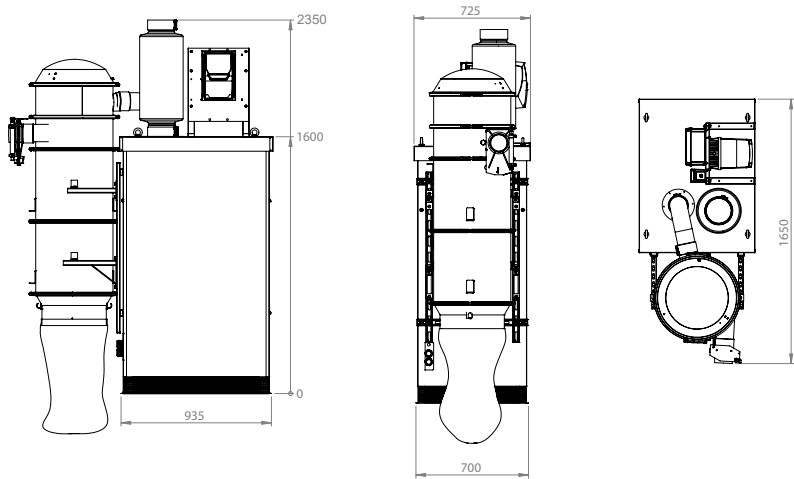
Dimensioner, installationsexempel, DC 11-Module XL
