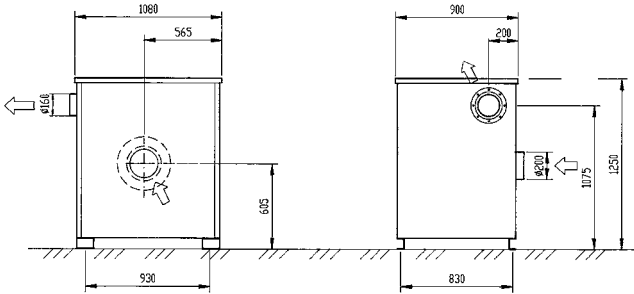
Dimensions RAF 1600 / 2500
