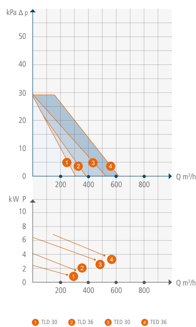
Turbopumparna TLD/TED
