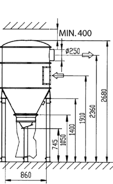
Dimensioner, installationsexempel F 30000
