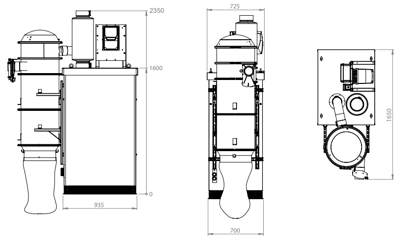
Dimensioner, installationsexempel, DC 11-Module XL
