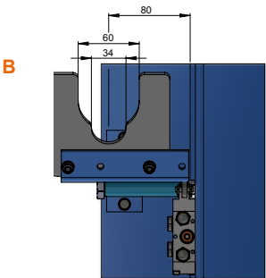
B Spring-loaded 5/2-valve (controls the shutter valve within the extraction system)
