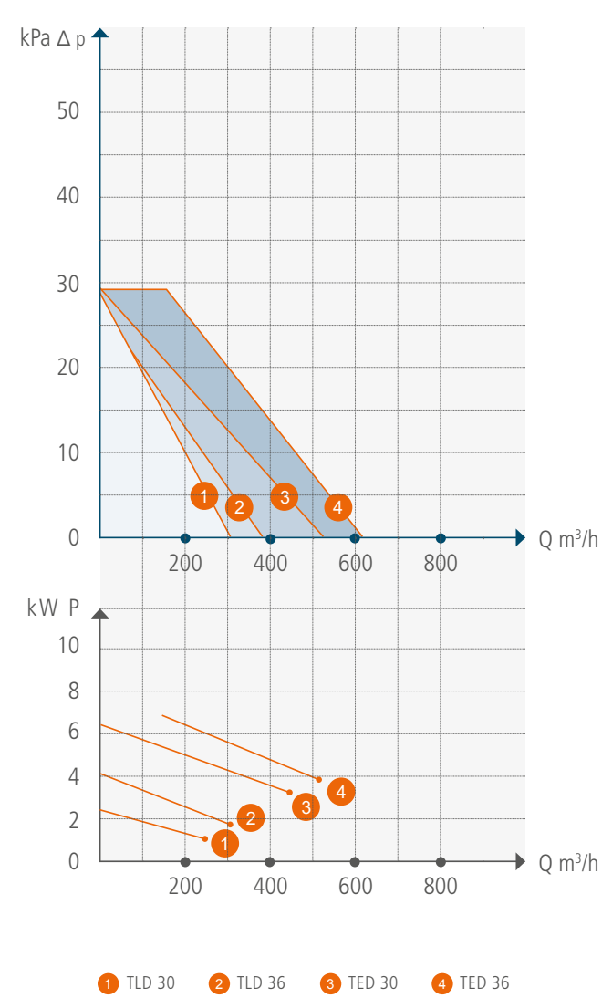
Turbopumps TLD/TED
