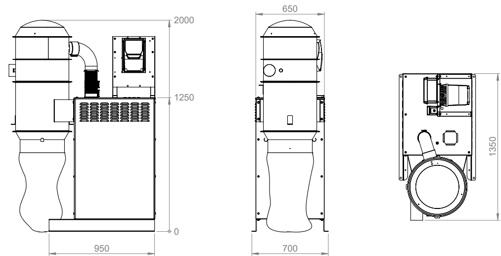
Dimensions, installation examples, DC 11-Module Standard
