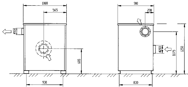
Dimensions RAF 1600 / 2500
